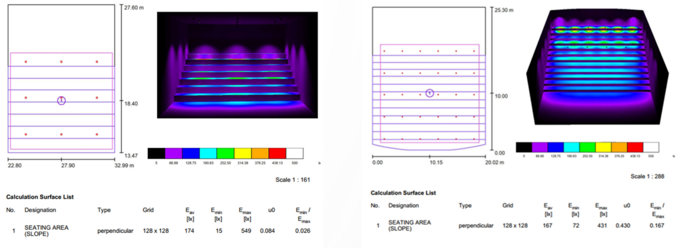
LUX Report showing the actual illuminance levels in the space.
